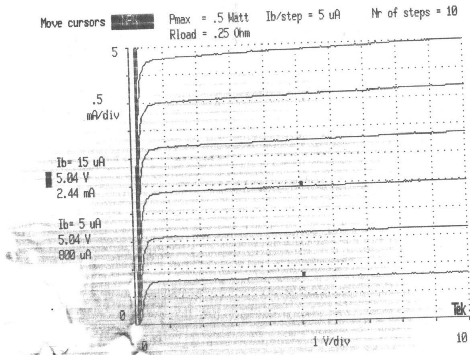
2N3904 and 2N3906 low current IV curves
