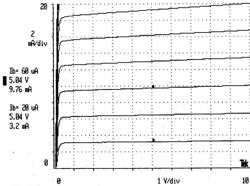
2N3904 and 2N3906 High current IV curves
